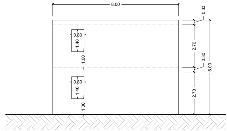
RIGHT-SIDE VIEW
